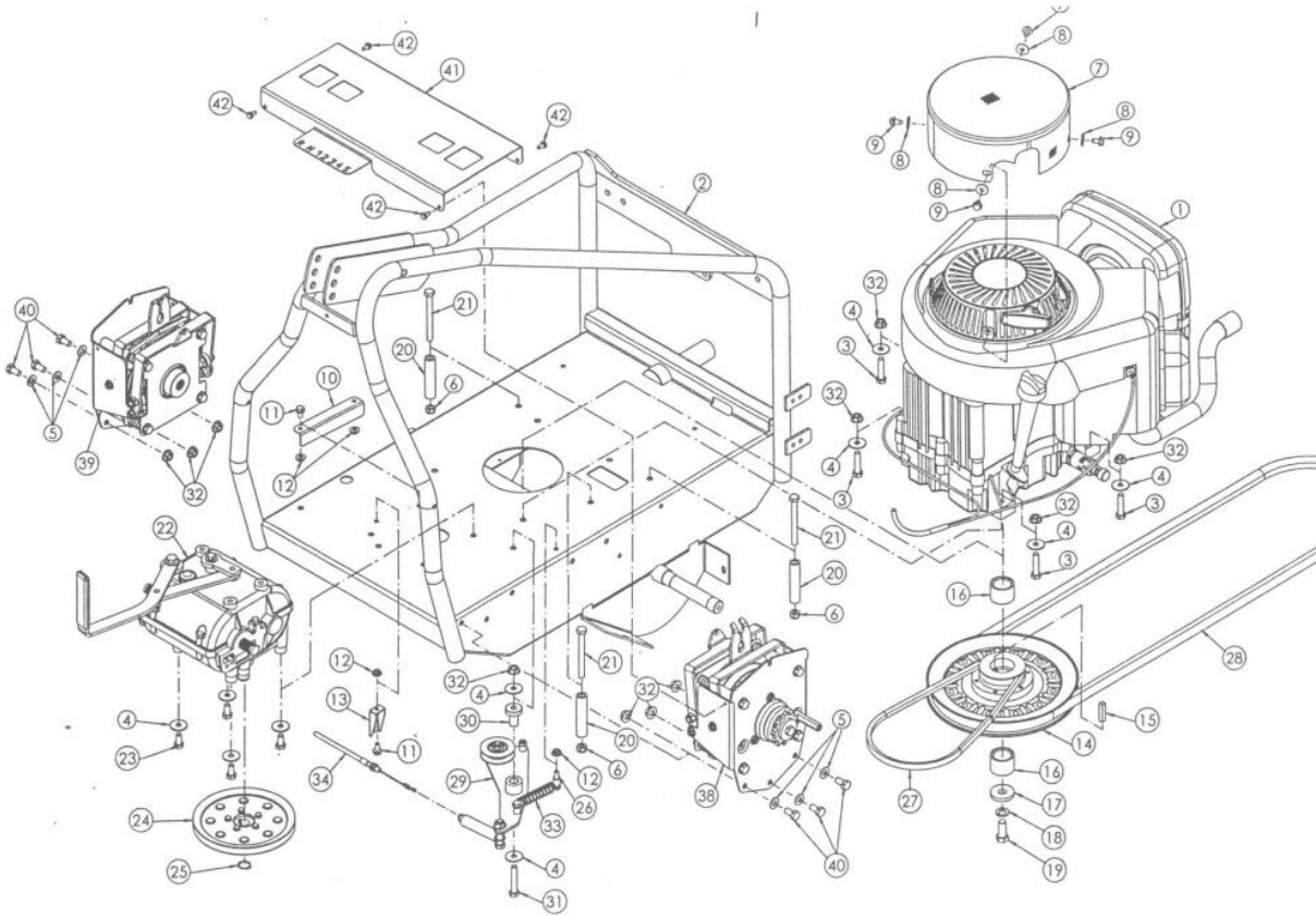
Fahrwerk AS 84 LB BI 03/2000
